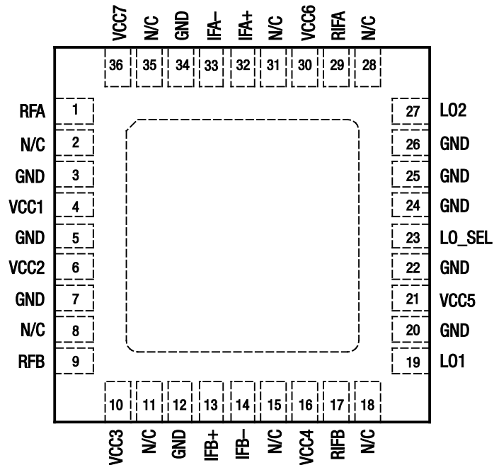
Figure 2. SKY73089-11 Pinout – 36-Pin MCM (Top View)
